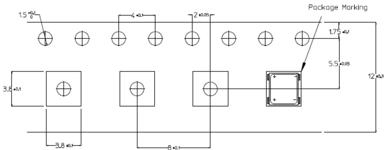
Carrier Tape
